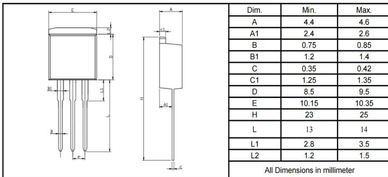
T0-262
