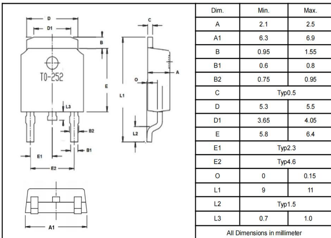
T0-252
