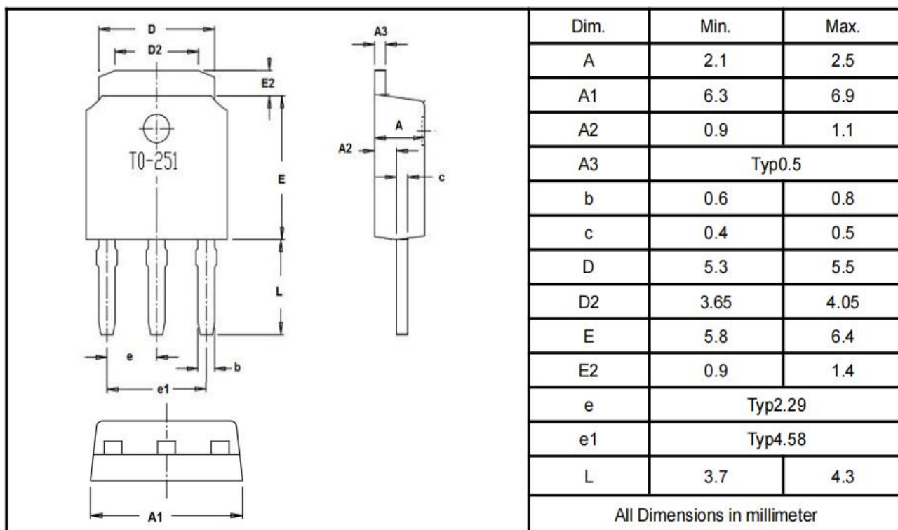
T0-251
